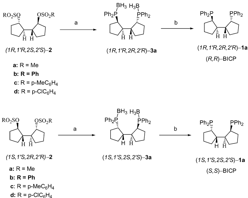
SCHEME 1 Synthesis of ( R,R )-BICP and ( S,S )-BICP. Reagents and conditions: a) NaOBu t /BuLi, Ar 2 PH(BH 3 ), 2b , toluene, 0°C to RT, 24 h, 50–51% yield; b) HBF 4 ·xOMe 2 , CH 2 Cl 2 , 0°C to RT, 24 h, >90% yield.
